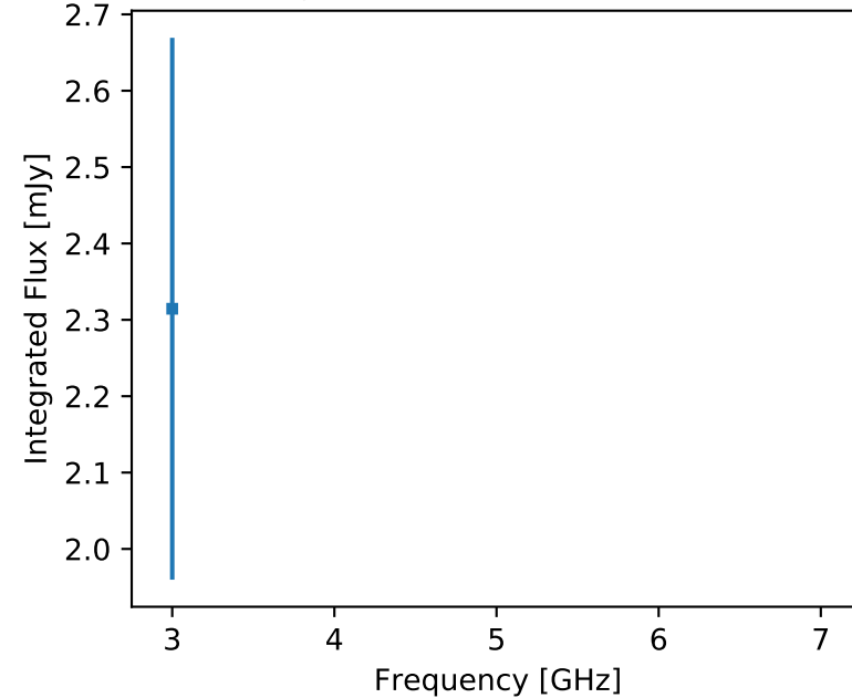
F357 J122058.79-274627.3 (unr)
