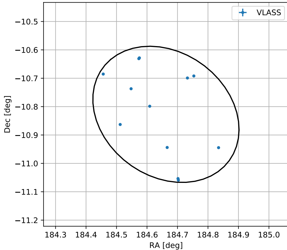
4FGL J1218.6-1049
