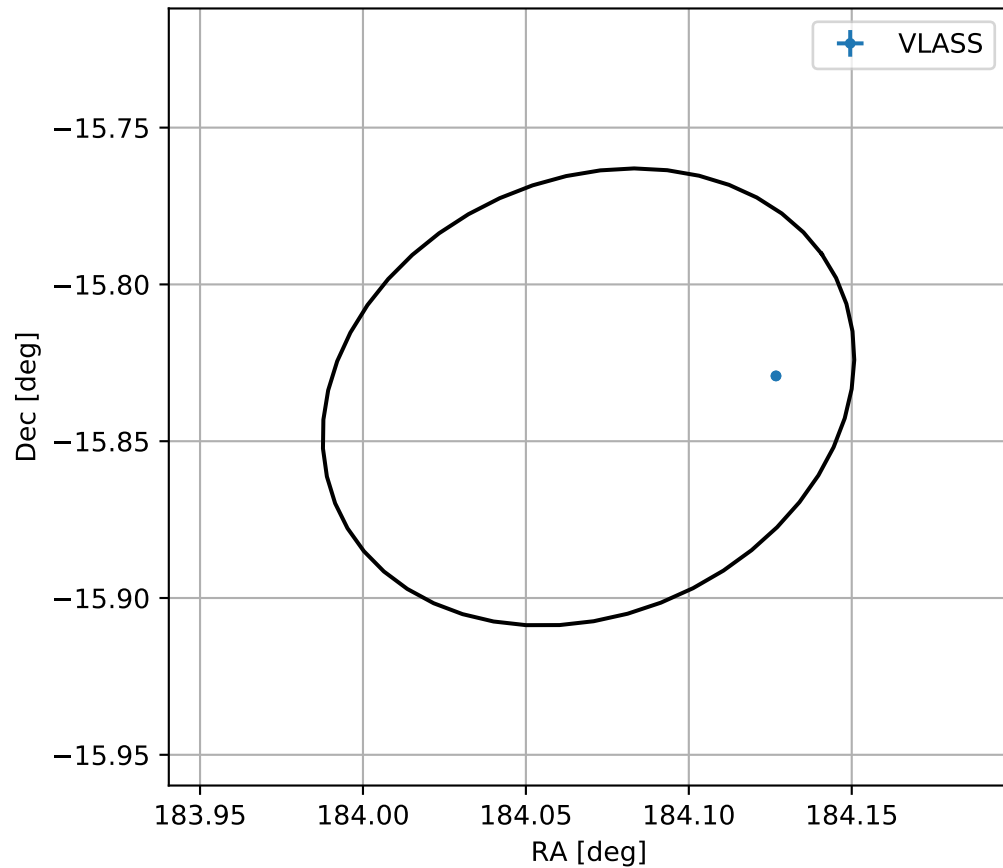
4FGL J1216.2-1550
