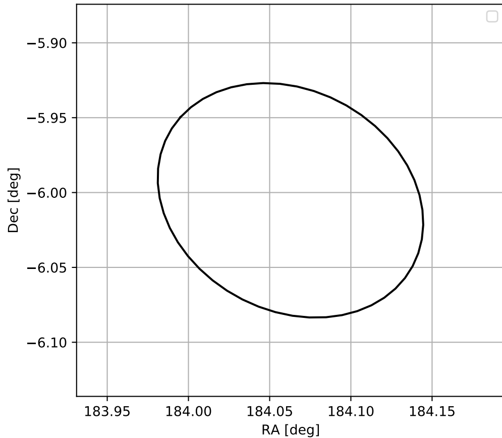
4FGL J1216.2-0600
