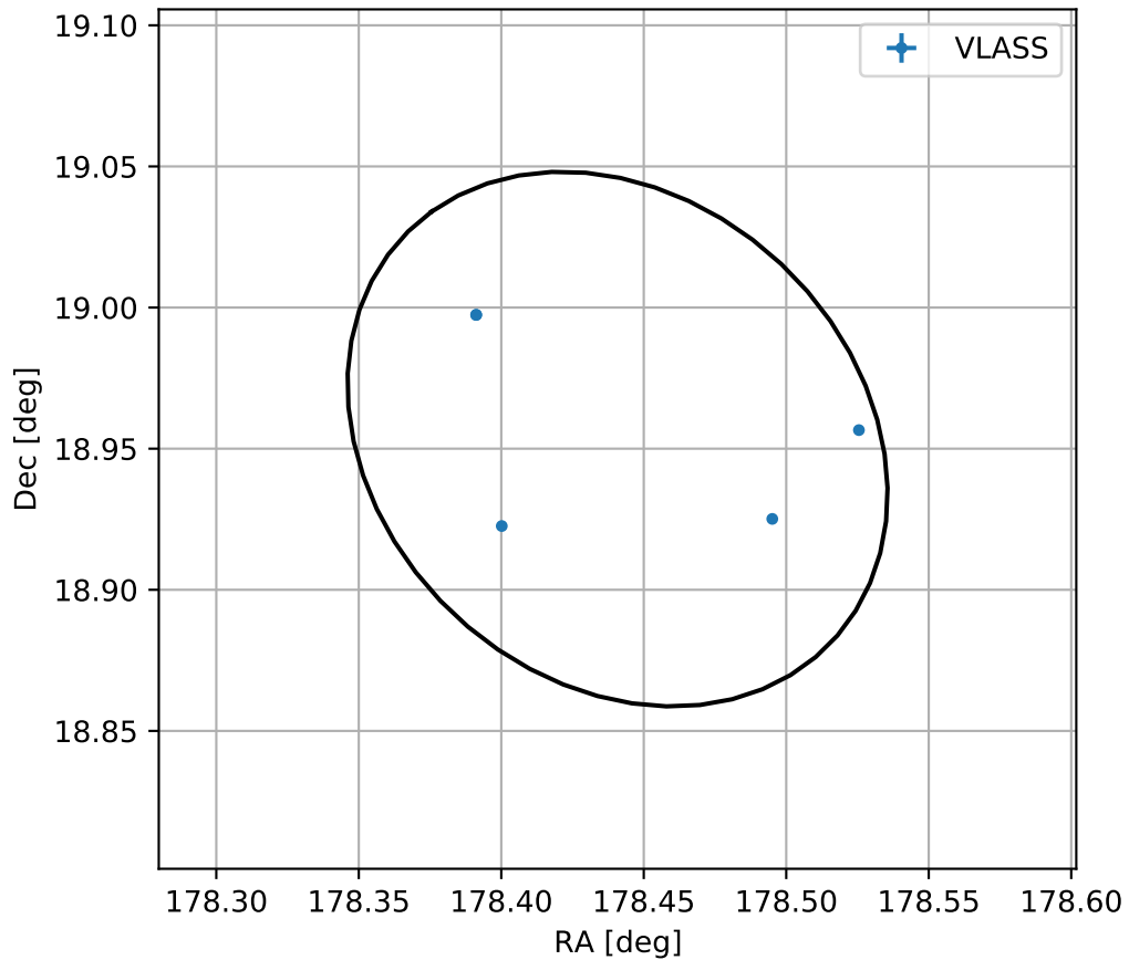
4FGL J1153.7+1857
