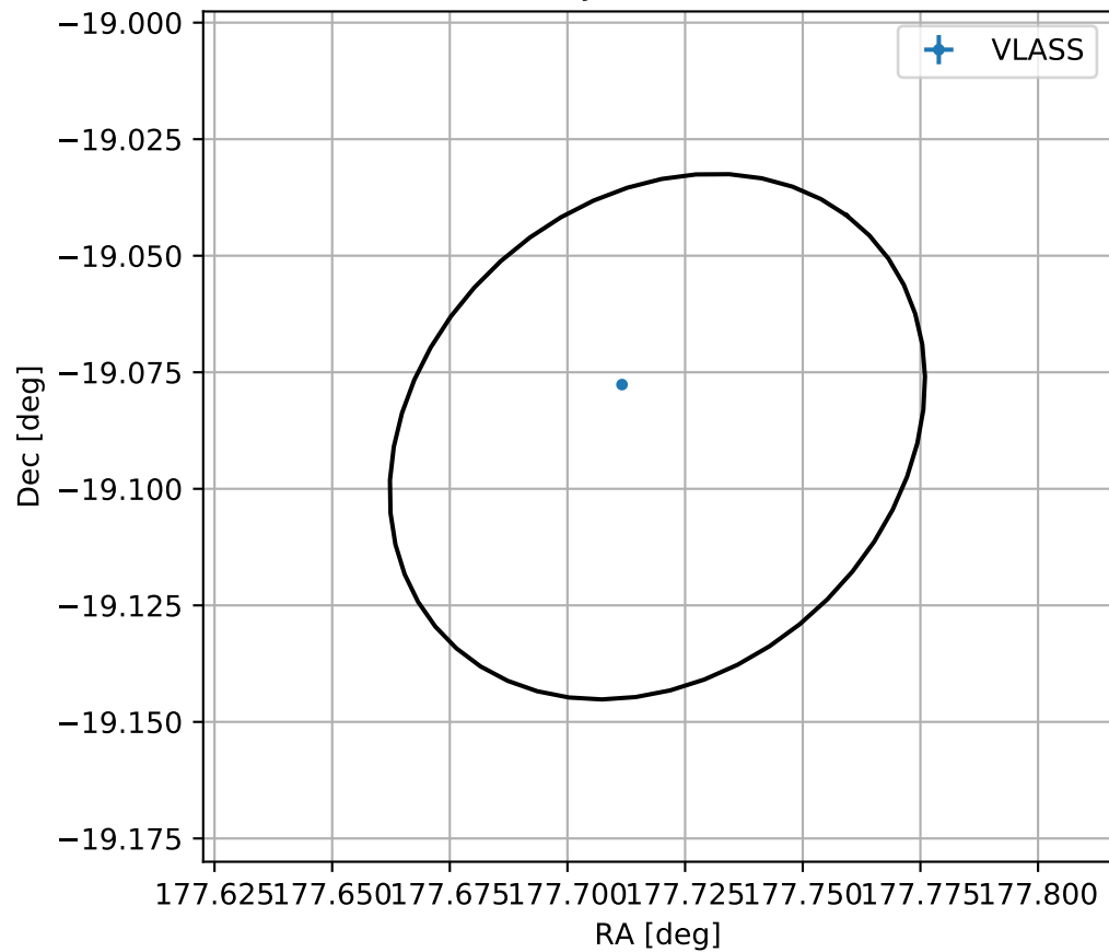
4FGL J1150.8-1905
