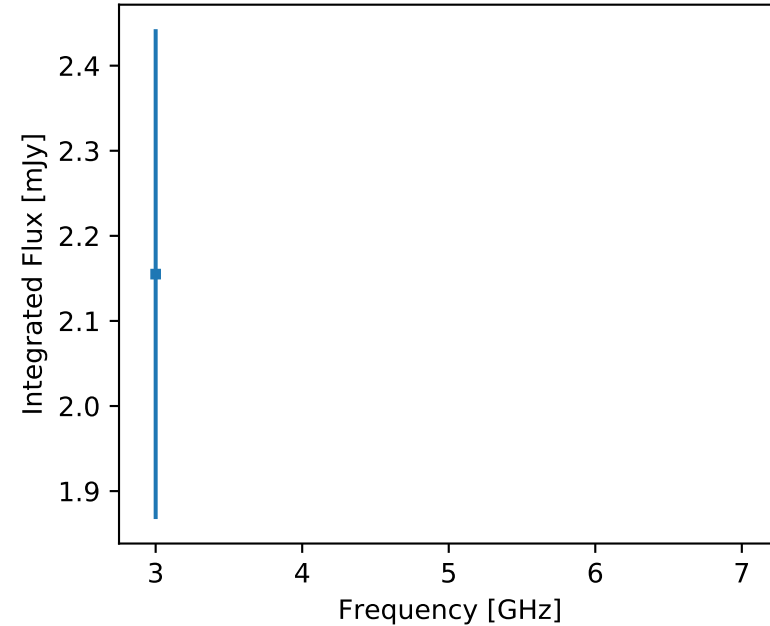
F357 J115050.78-190439.5 (unr)
