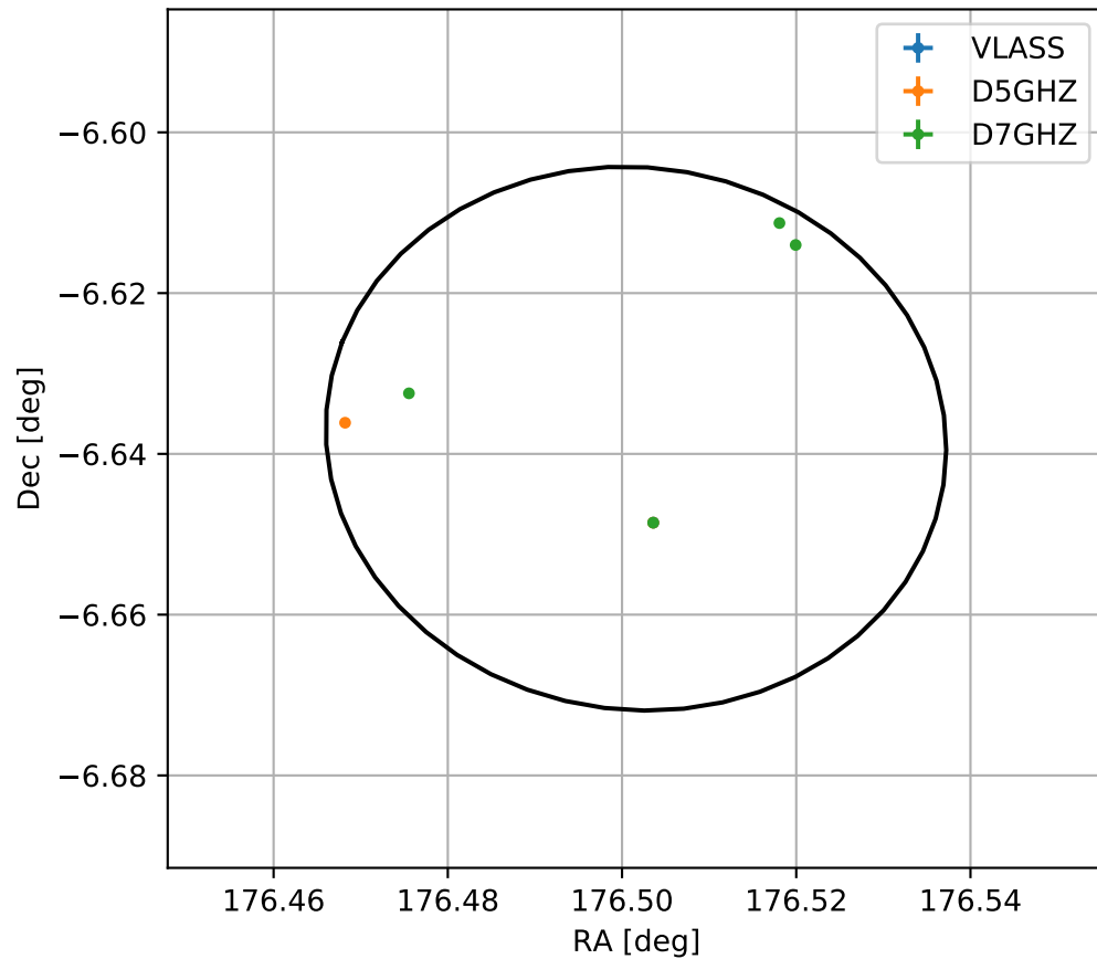
4FGL J1146.0-0638
