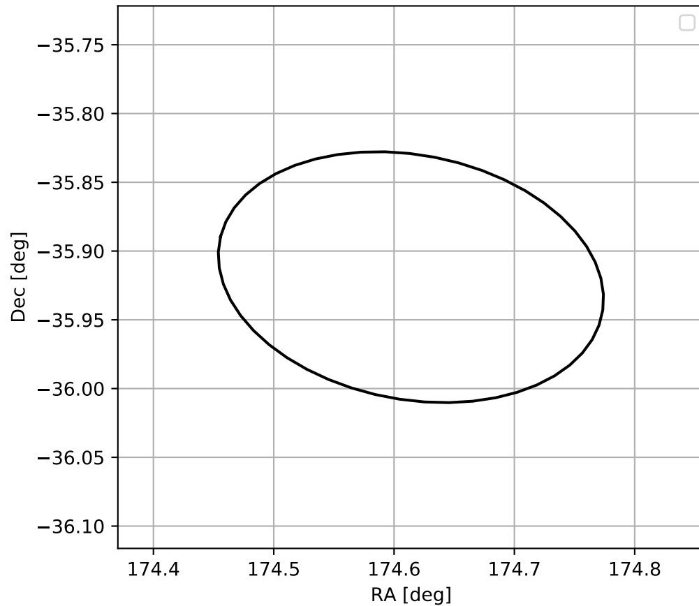
4FGL J1138.4-3555
