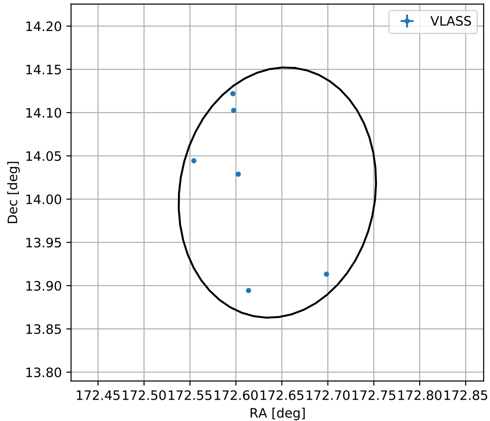
4FGL J1130.5+1400
