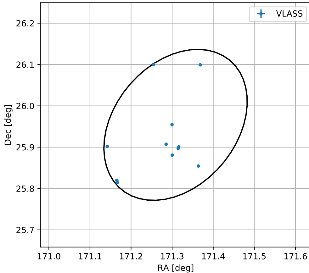
4FGL J1125.2+2557
