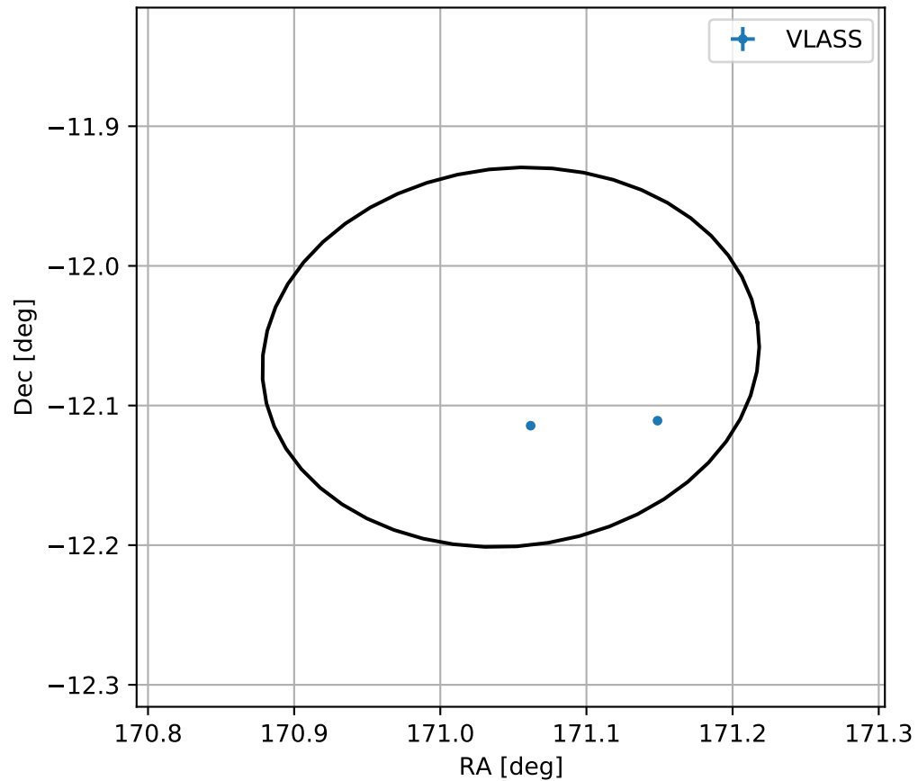
4FGL J1124.1-1203
