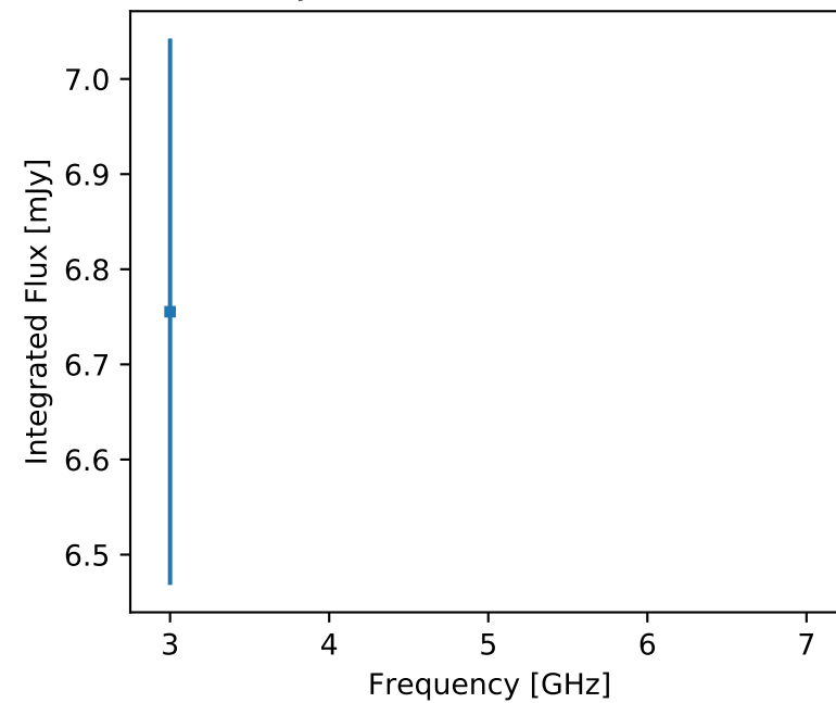
F357 J112435.67-120639.1 (unr)
