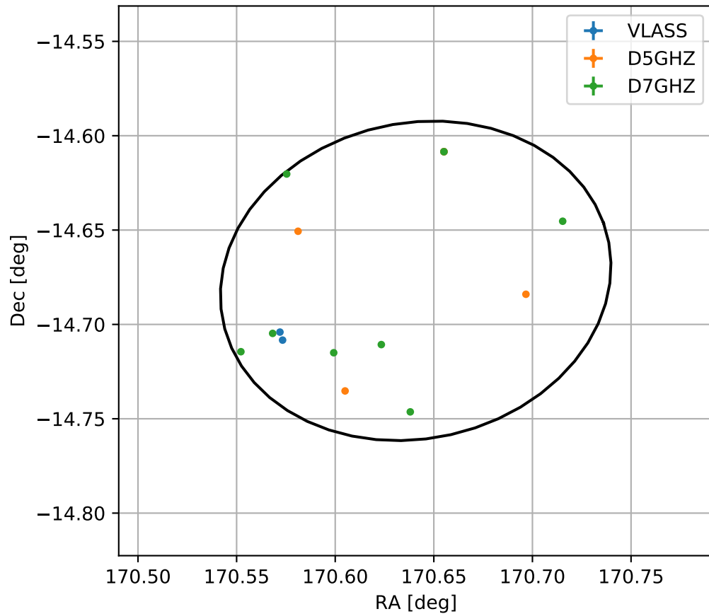
4FGL J1122.5-1440
