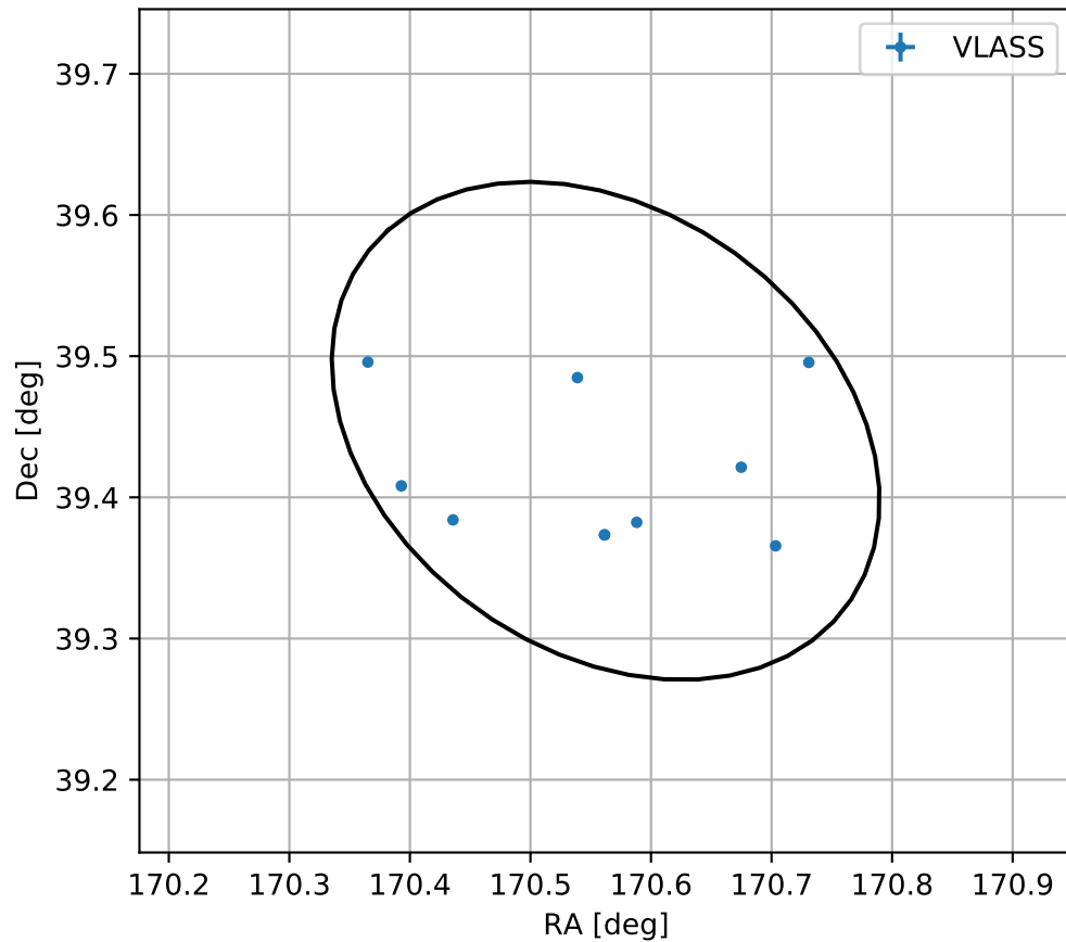
4FGL J1122.2+3926
