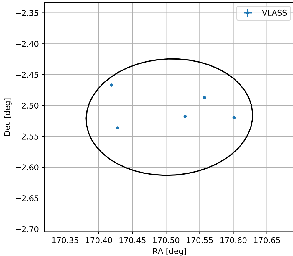
4FGL J1122.0-0231
