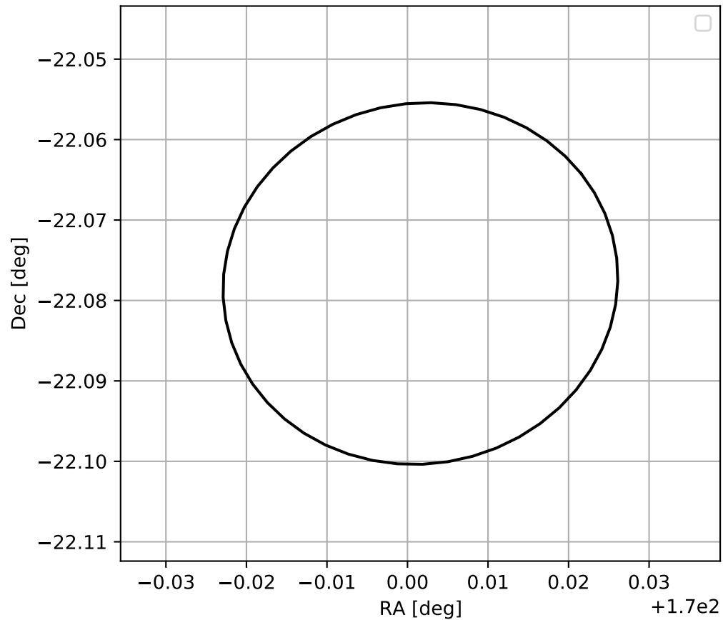
4FGL J1120.0-2204
