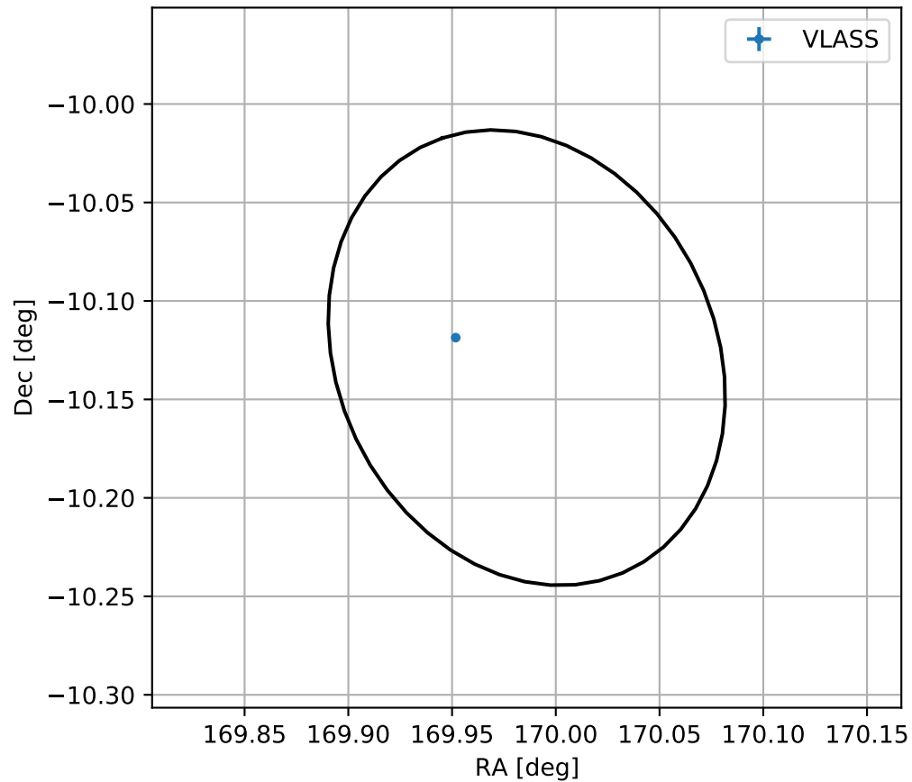
4FGL J1119.9-1007
