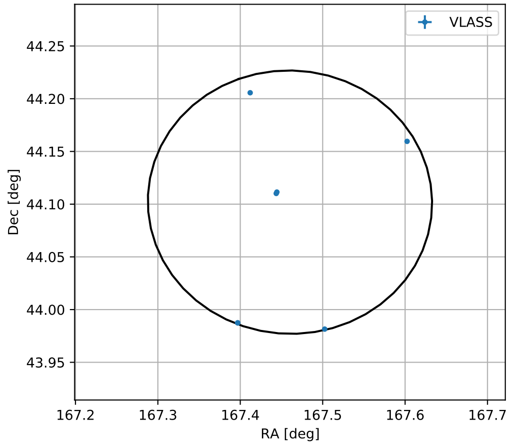
4FGL J1109.8+4406
