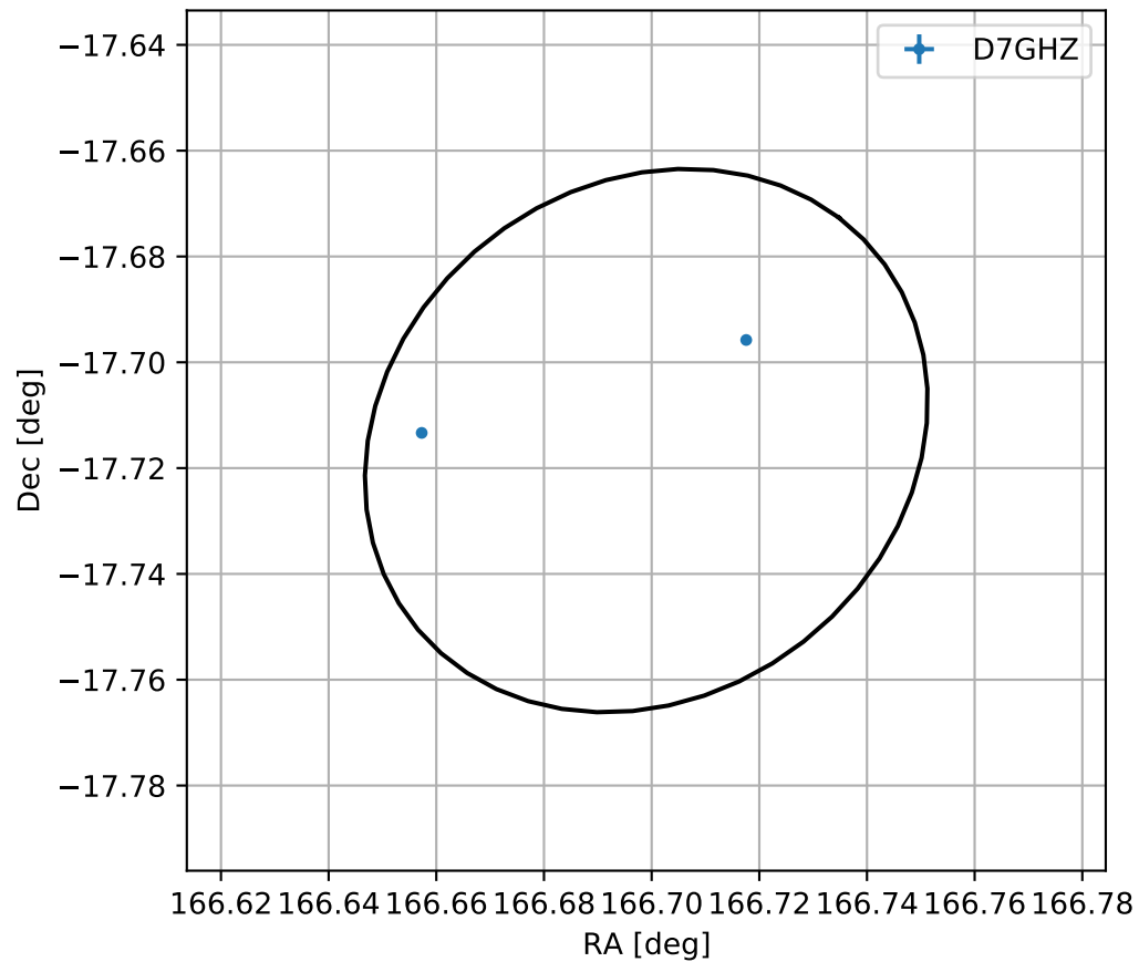
4FGL J1106.7-1742
