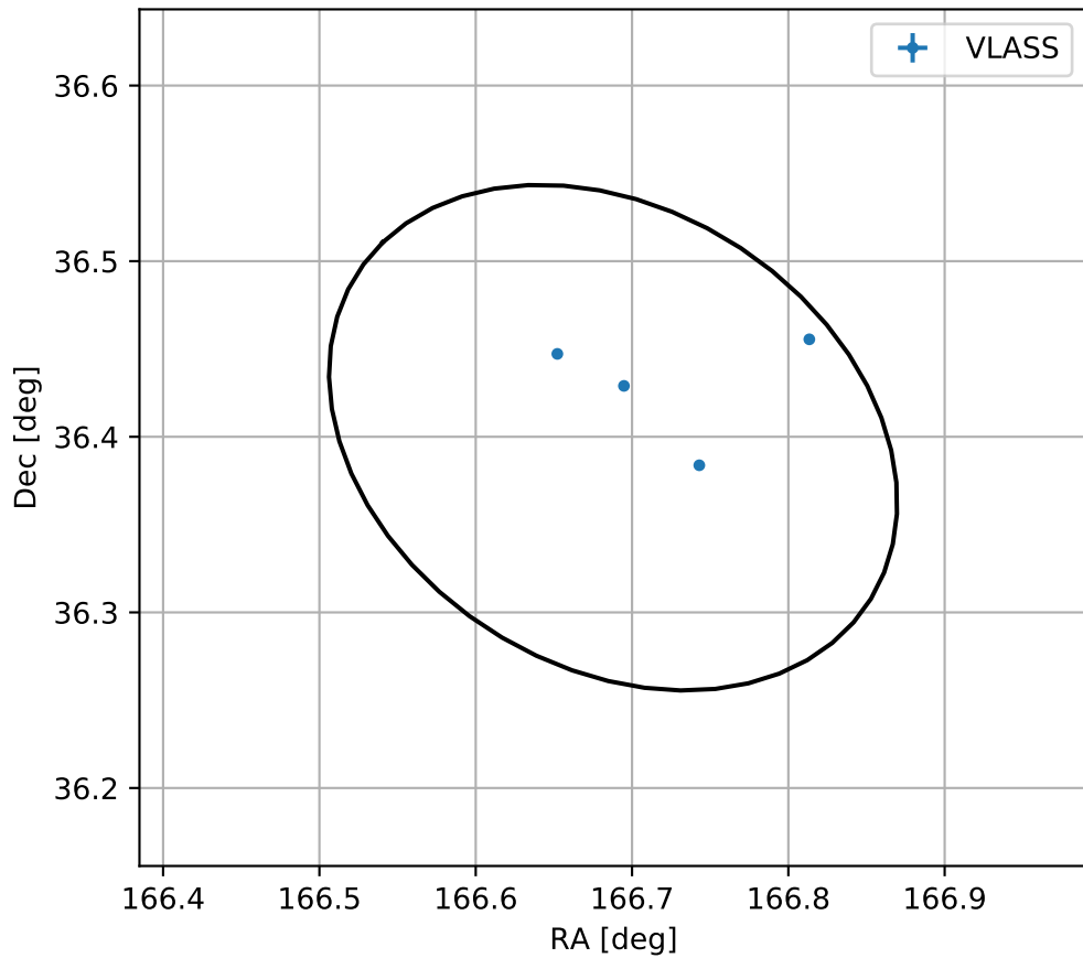
4FGL J1106.7+3623
