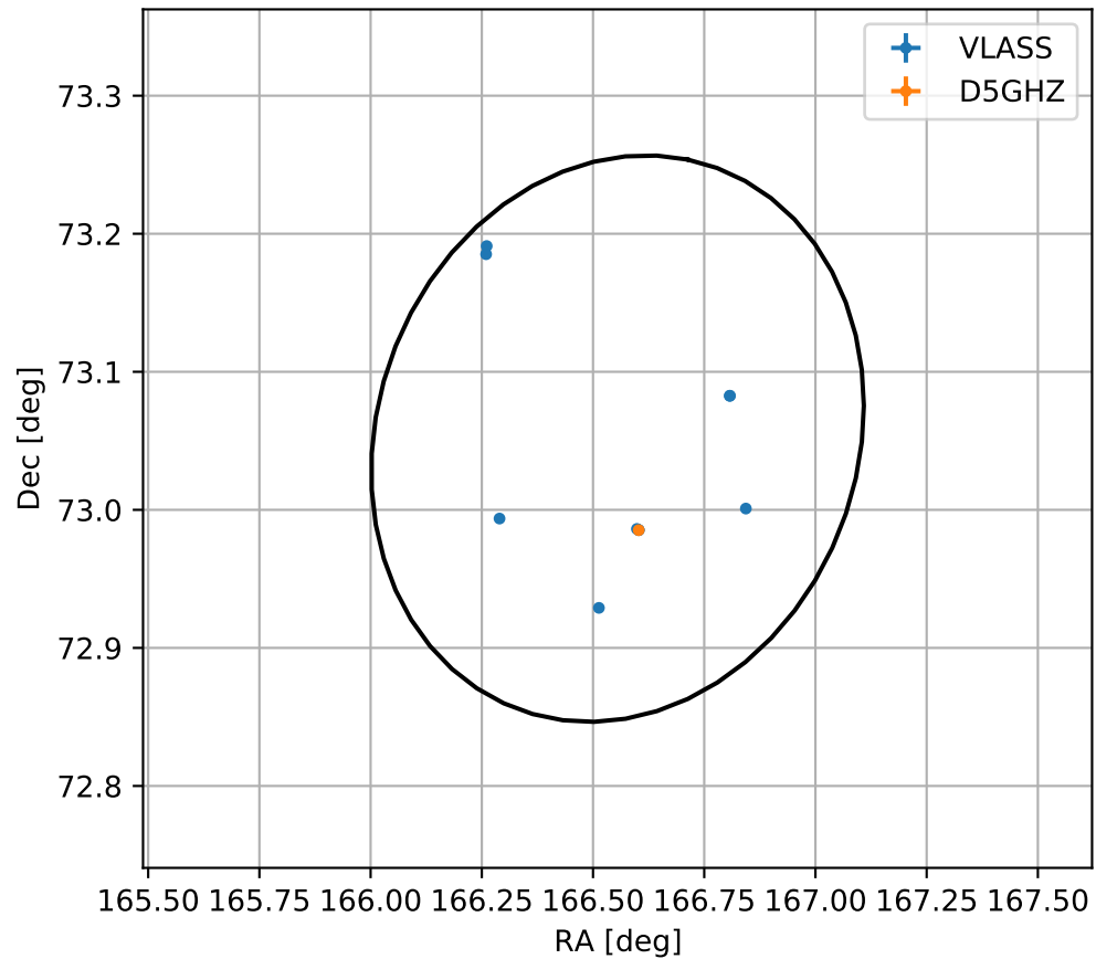
4FGL J1106.2+7303
