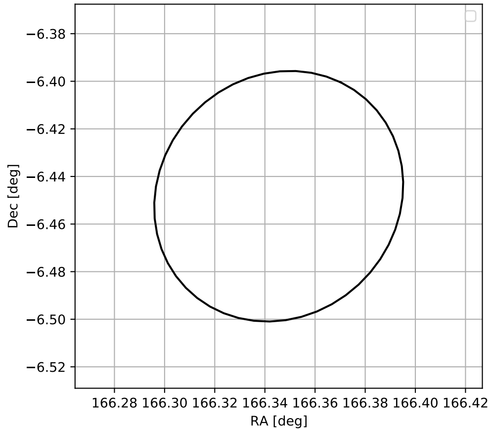
4FGL J1105.3-0626
