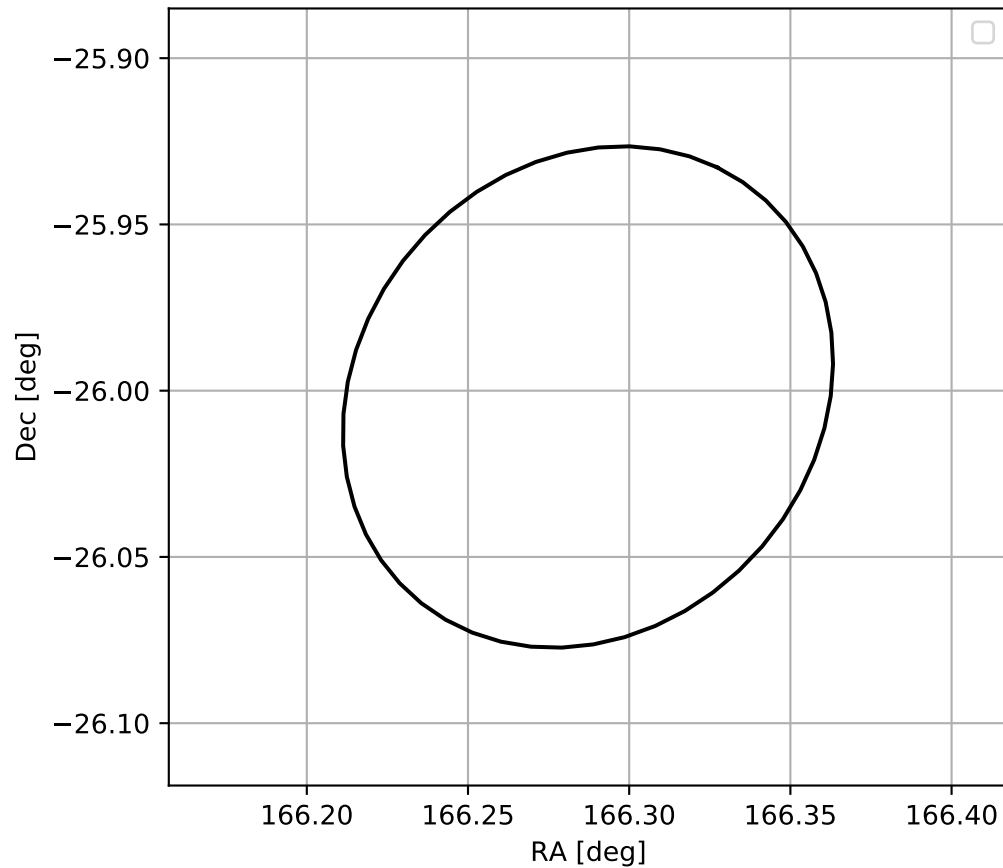
4FGL J1105.1-2600
