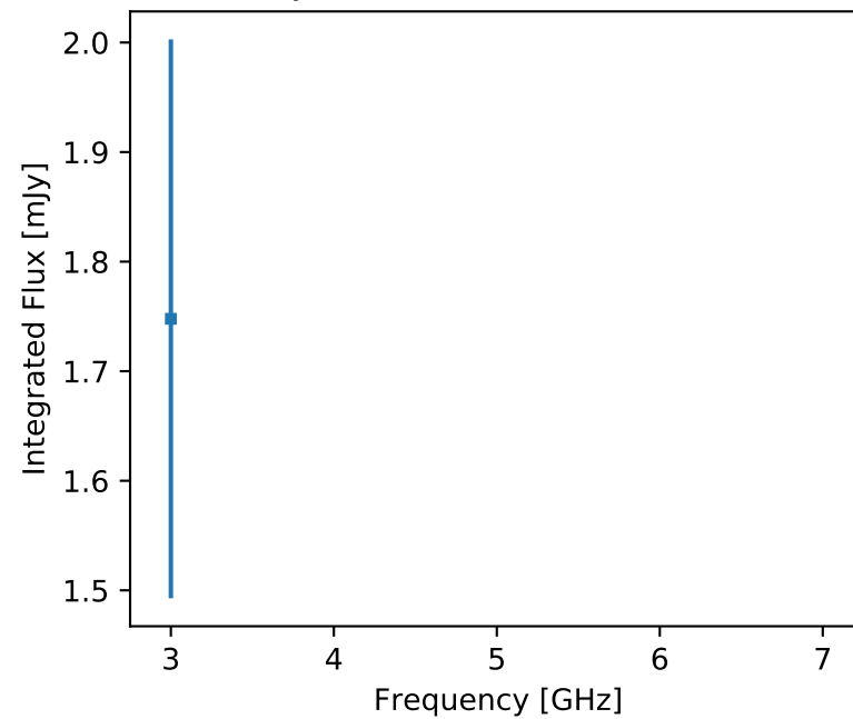
F357 J110236.37+025300.5 (unr)
