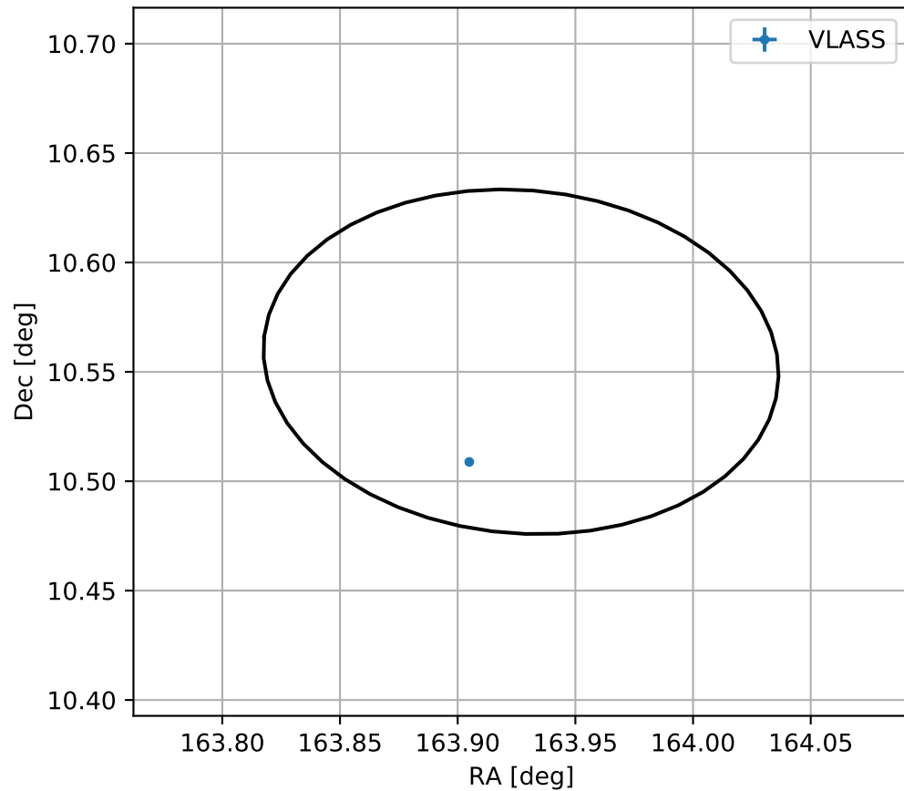
4FGL J1055.7+1033
