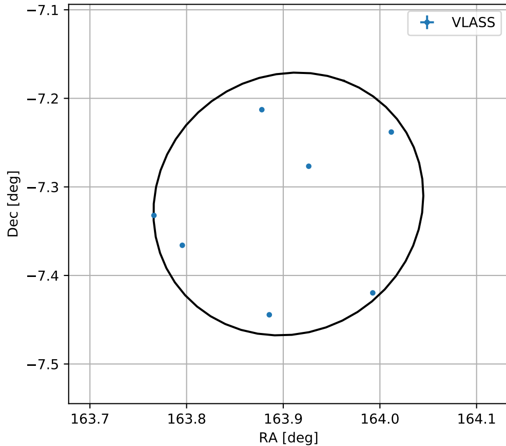
4FGL J1055.6-0719
