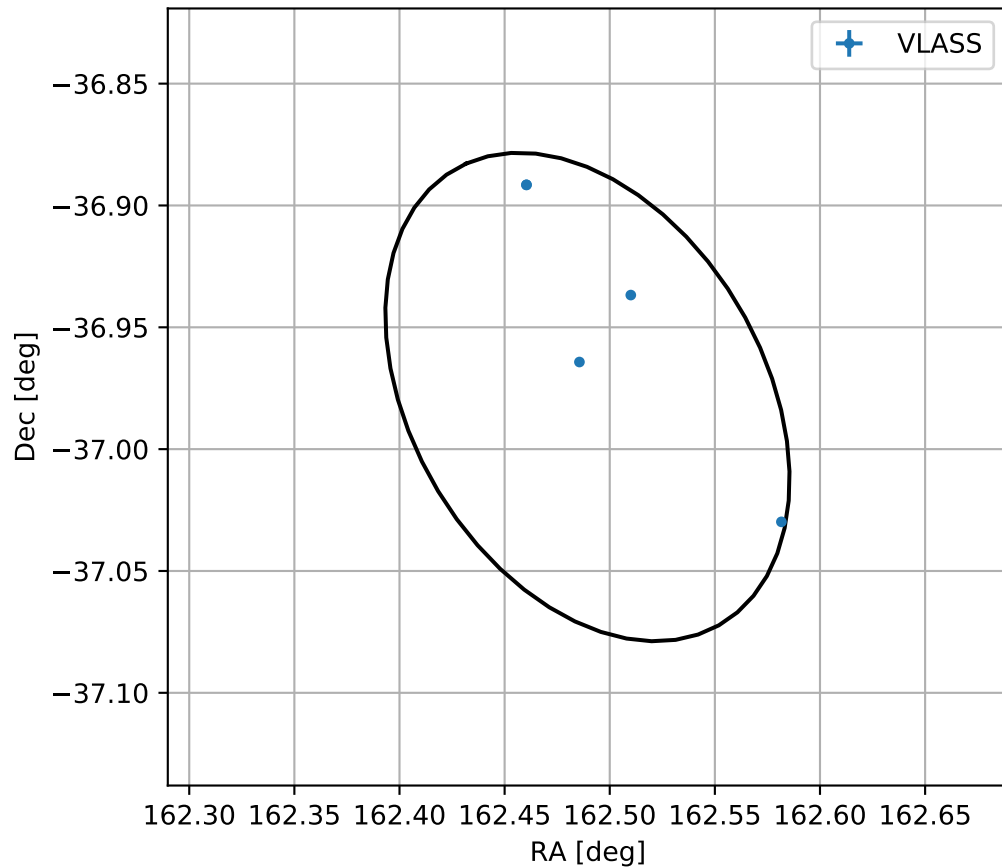
4FGL J1049.9-3658
