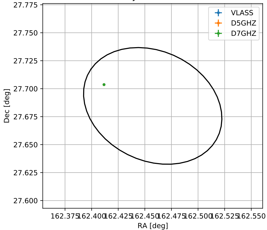
4FGL J1049.8+2741
