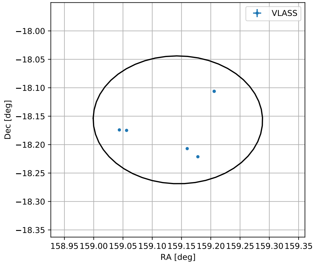
4FGL J1036.5-1809
