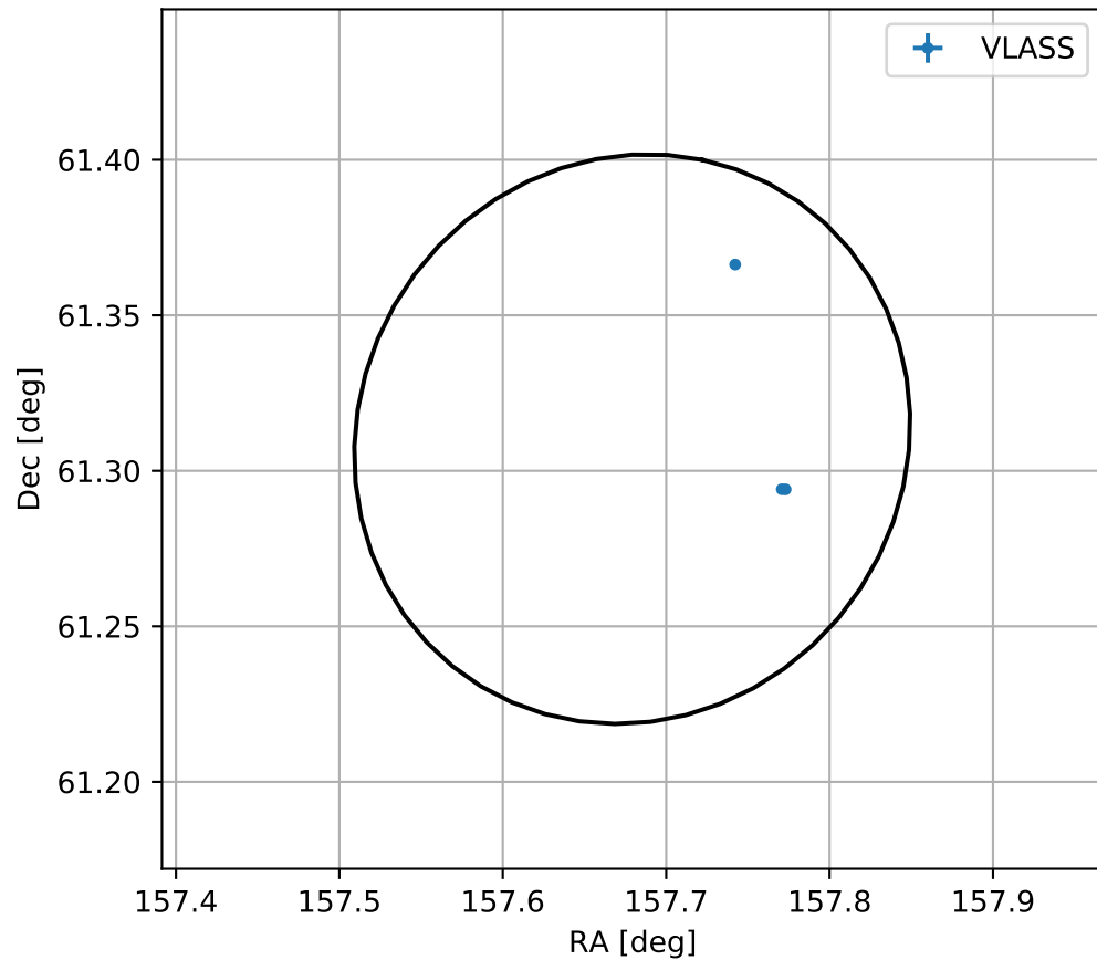
4FGL J1030.7+6118
