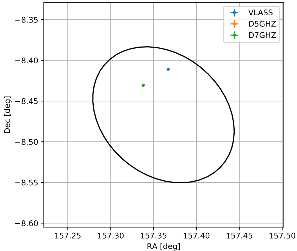
4FGL J1029.4-0828
