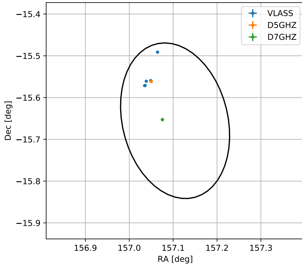
4FGL J1028.4-1539
