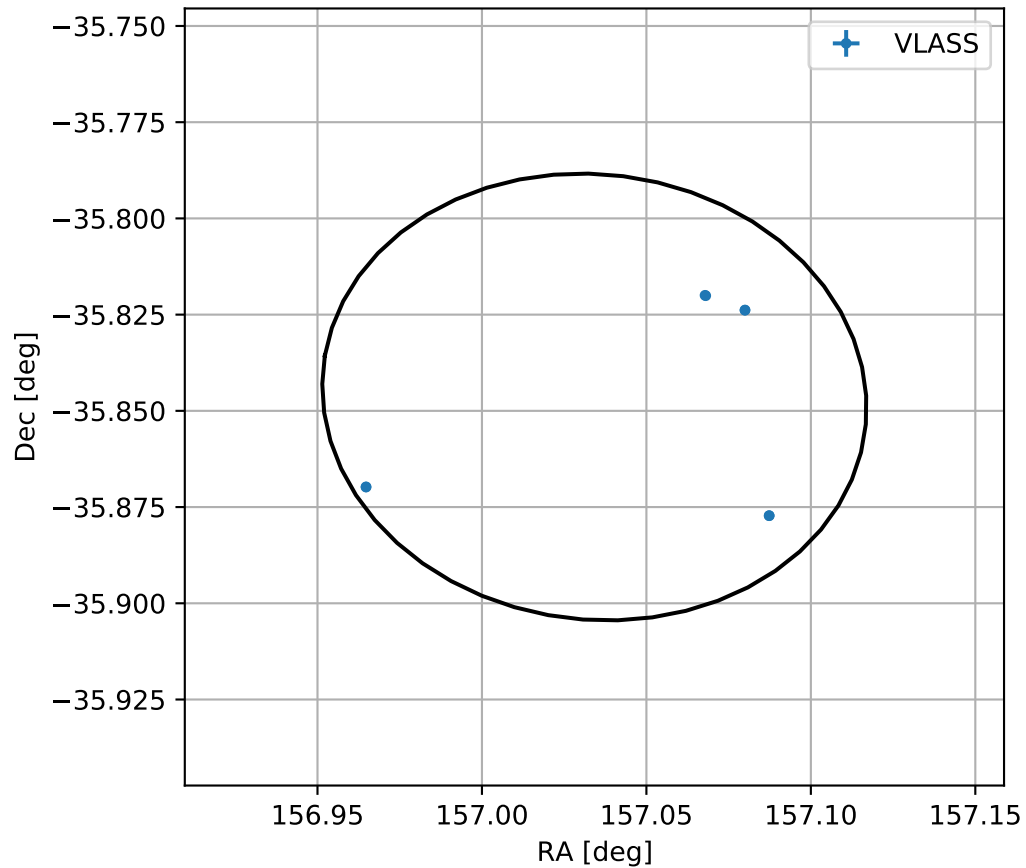
4FGL J1028.1-3550
