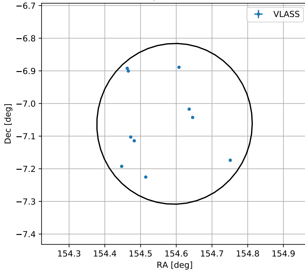
4FGL J1018.3-0703
