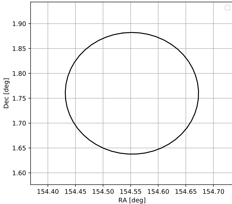
4FGL J1018.2+0145
