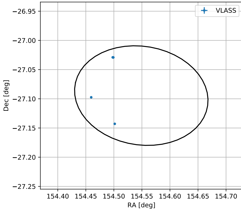
4FGL J1018.1-2705
