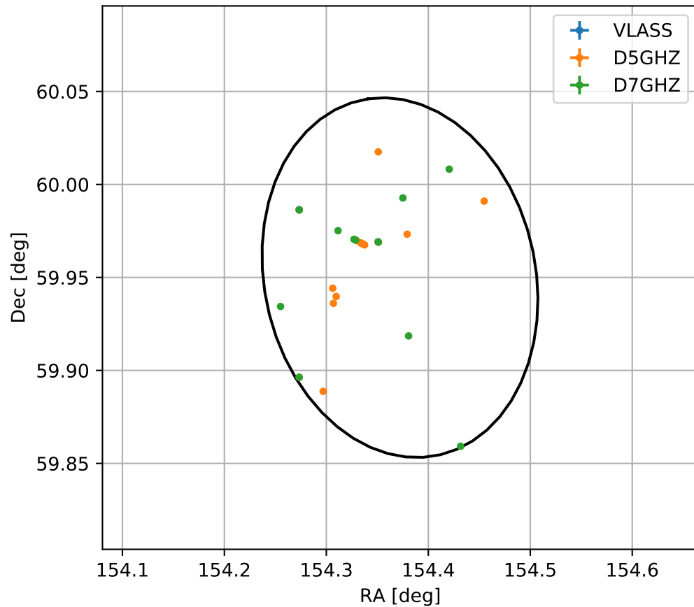
4FGL J1017.4+5956
