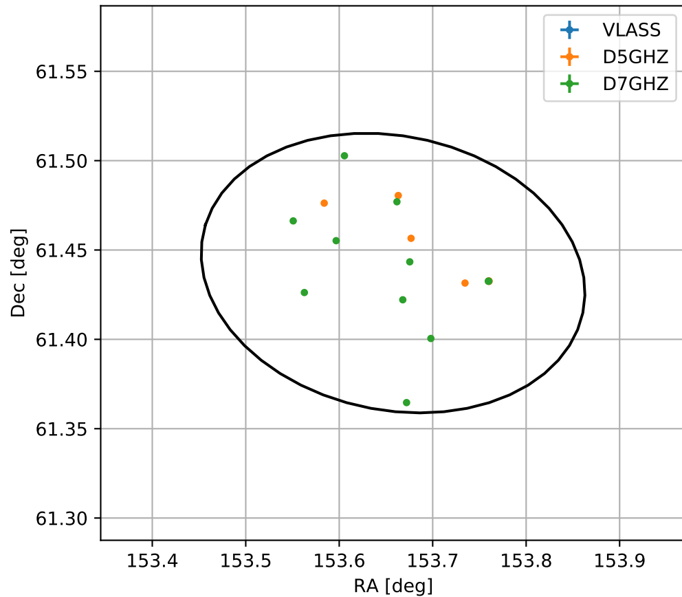
4FGL J1014.6+6126
