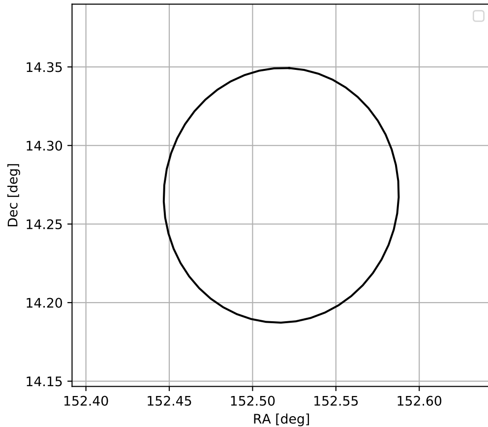
4FGL J1010.0+1416
