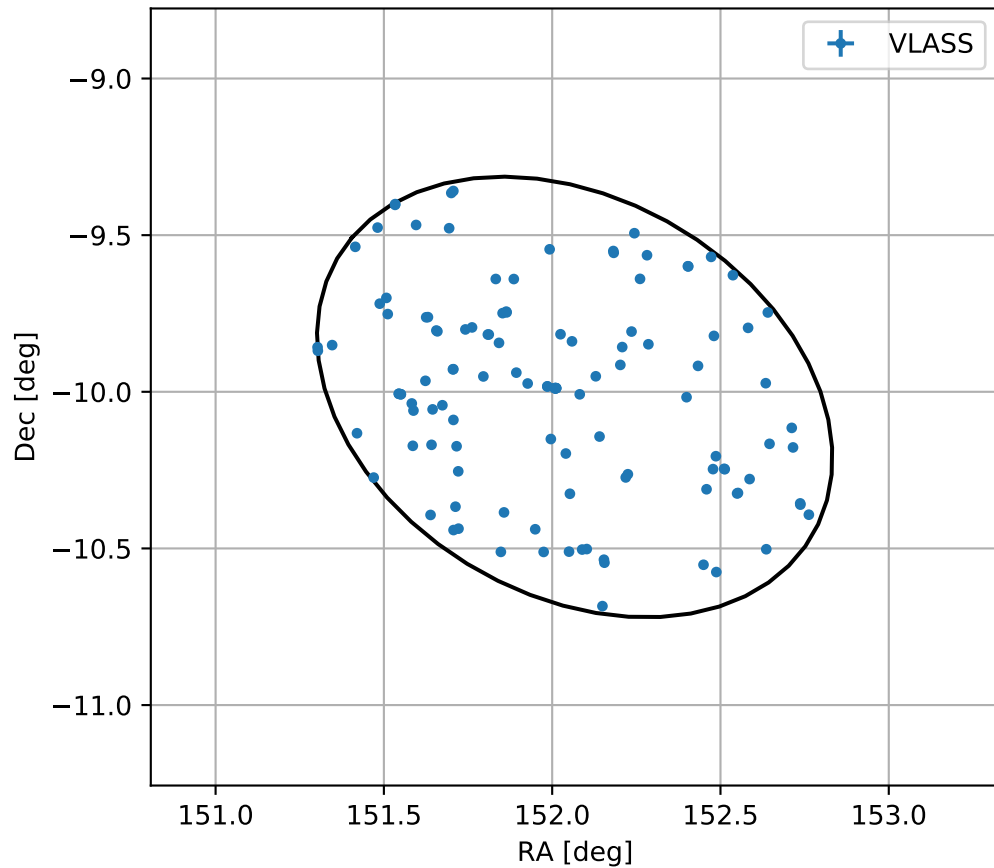
4FGL J1008.2-1000
