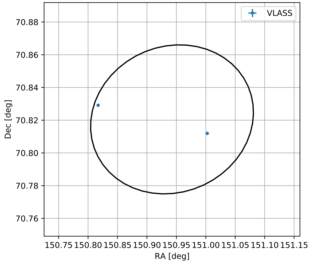
4FGL J1003.7+7049
