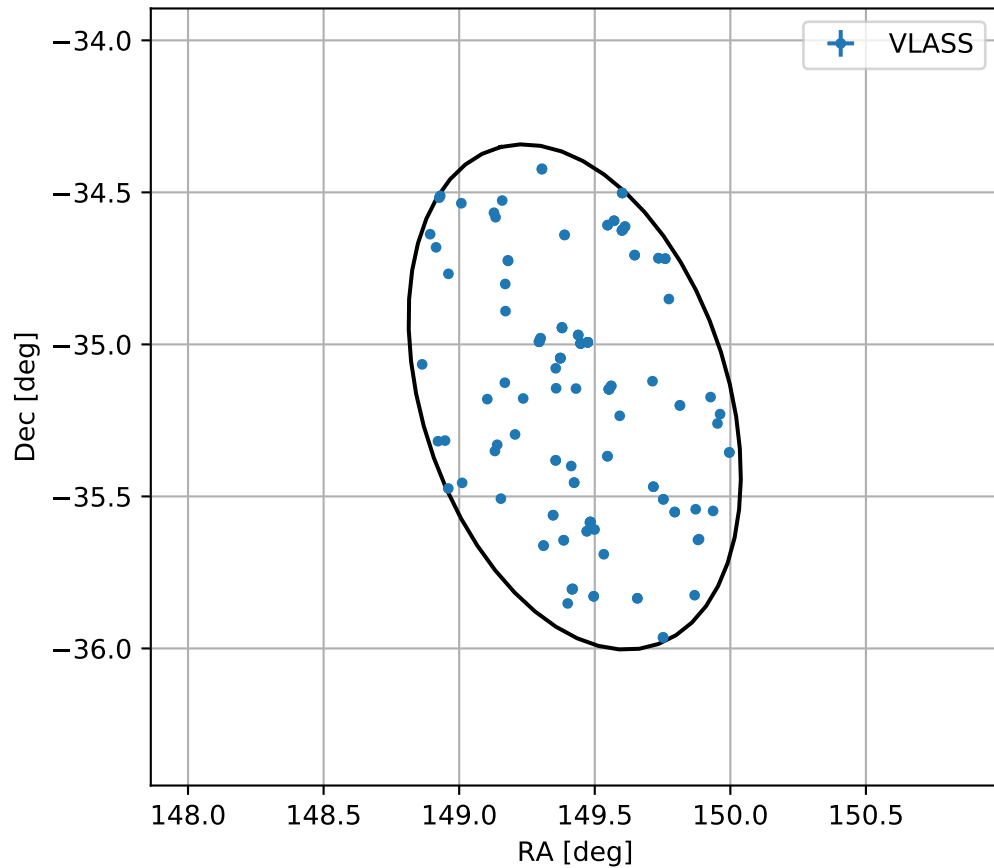
4FGL J0957.7-3510
