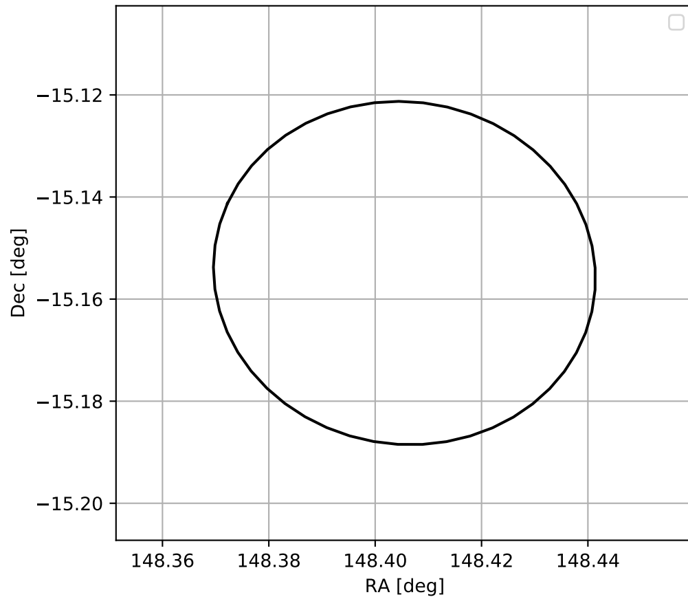
4FGL J0953.6-1509
