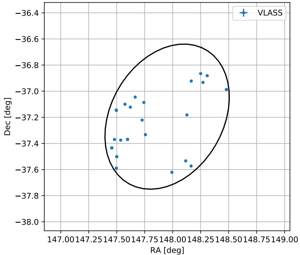
4FGL J0951.8-3711
