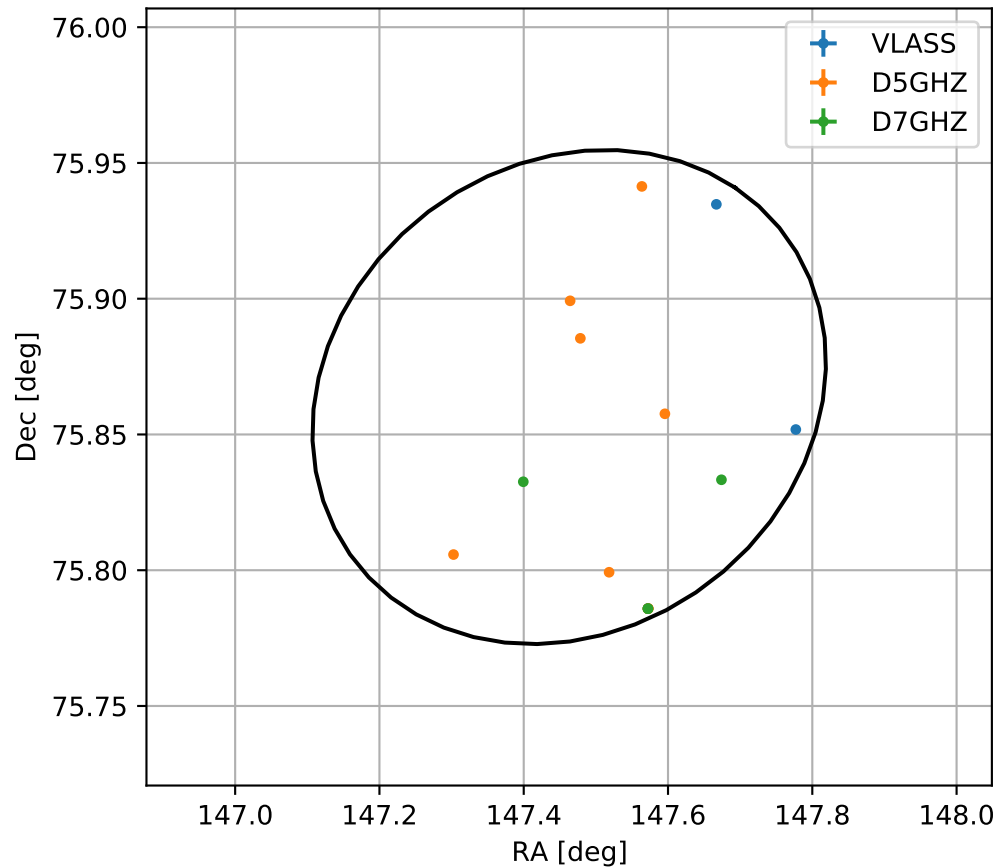
4FGL J0949.8+7551
