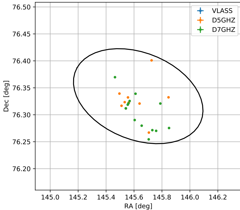
4FGL J0942.5+7620
