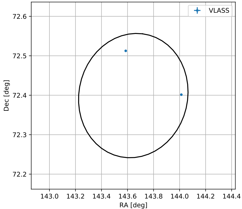
4FGL J0934.5+7223
