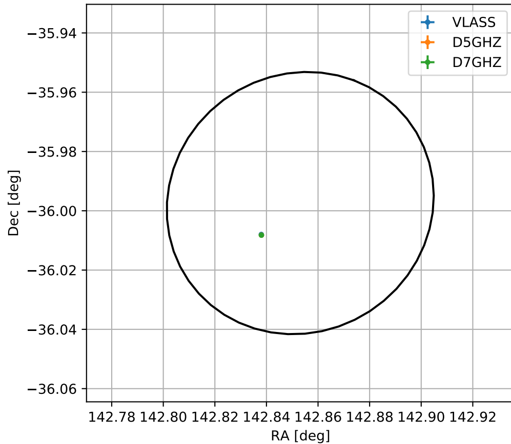
4FGL J0931.4-3559
