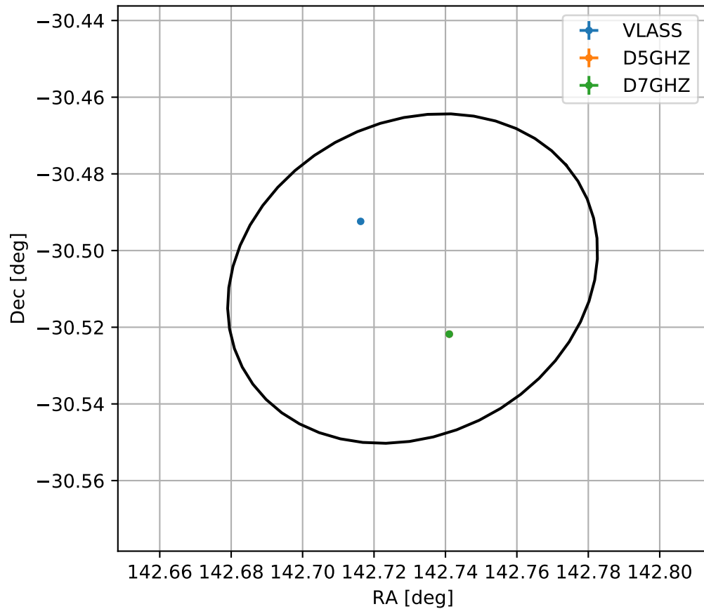
4FGL J0930.9-3030
